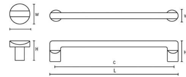
1482 ZINC Optional Finish: CP / MBB / BN / PB / MB
